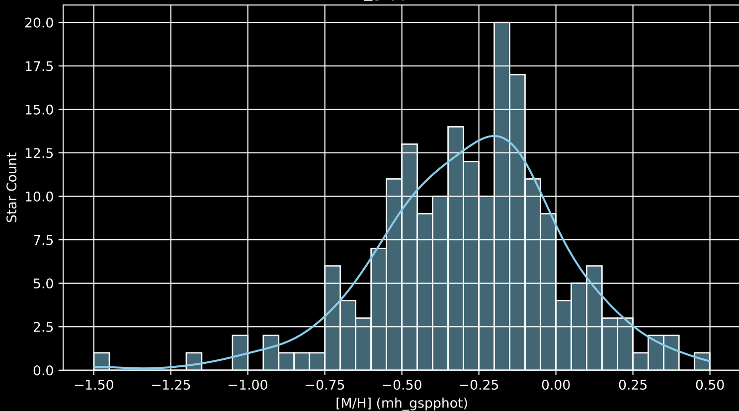
APOGEE DR17 Field: [K2_C3_045-47 [M/H] (mh_gspphot) (n= 192)
