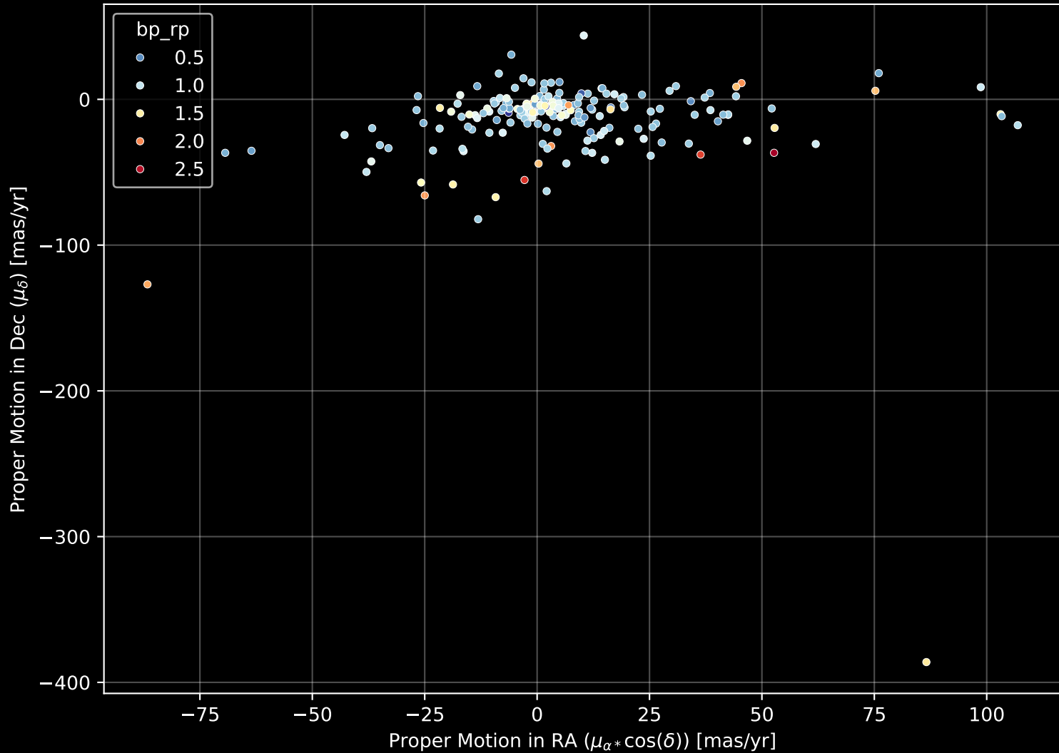
APOGEE DR17 Field: [K2_C3_045-47] Proper Motion Diagram (n= 193)
