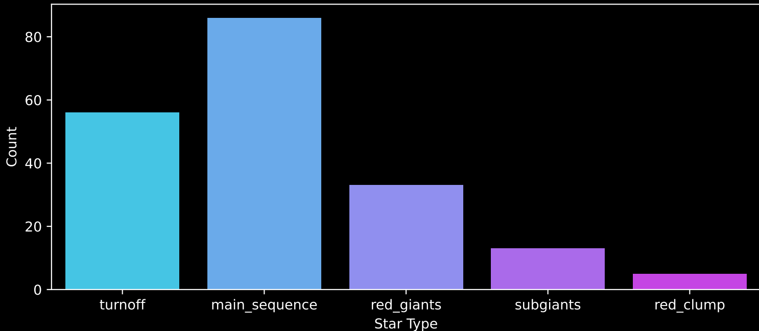
APOGEE DR17 Field: [K2_C3_045-47] Count plot of Star Type
