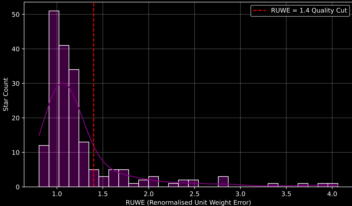
GAPOGEE DR17 Field [K2_C3_045-47] RUWE Distribution (n= 187)
