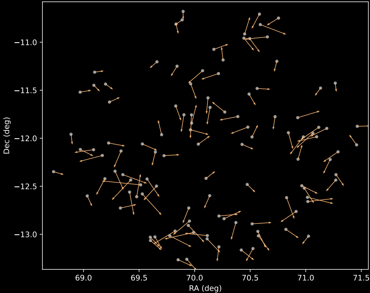
APOGEE DR17 Cluster 3 Proper Motion Vectors (n=111)
