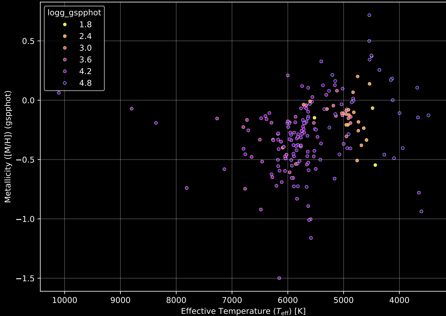
APOGEE DR17 Field: [K2_C3_045-47] Stellar Population Parameters (n= 193)
