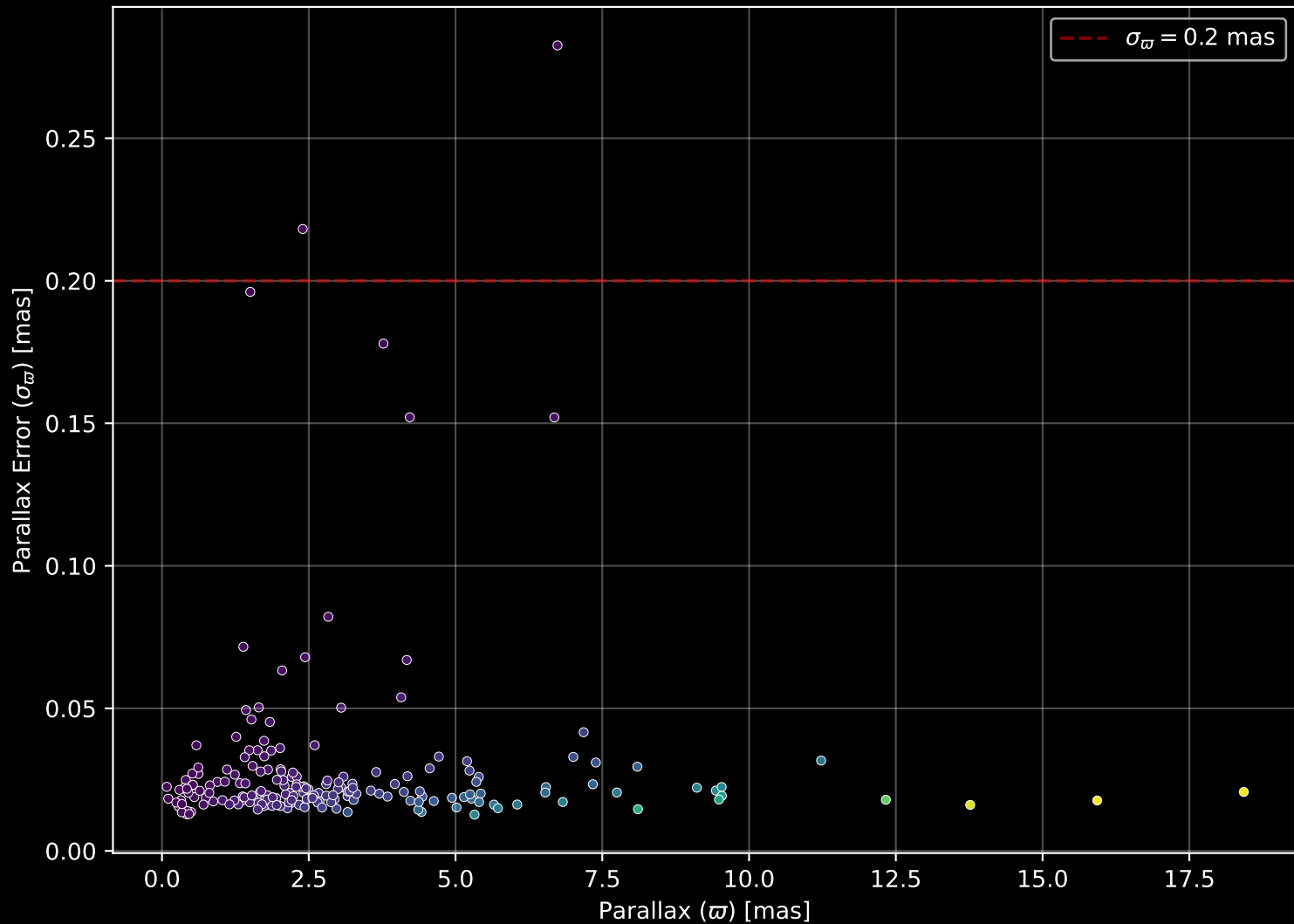
APOGEE DR17 Field: [K2_C3_045-47] Parallax Quality (n= 193)
